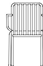
ARM CHAIR W51 x D56 x H80 cm Seat height 45 cm, Seat depth 41 cm Stackable 8 pcs.
