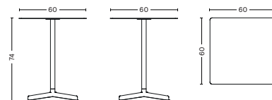
L60 x W60 x H74 cm
