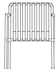
DINING ARM CHAIR W63 x D66 x H80 cm Seat height 45 cm, Seat depth 44 cm
